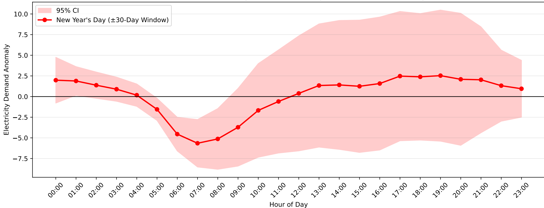
Pennant Hills Demand Anomaly: New Year's Day (2004–2017, \pm 30 -Day Window)
